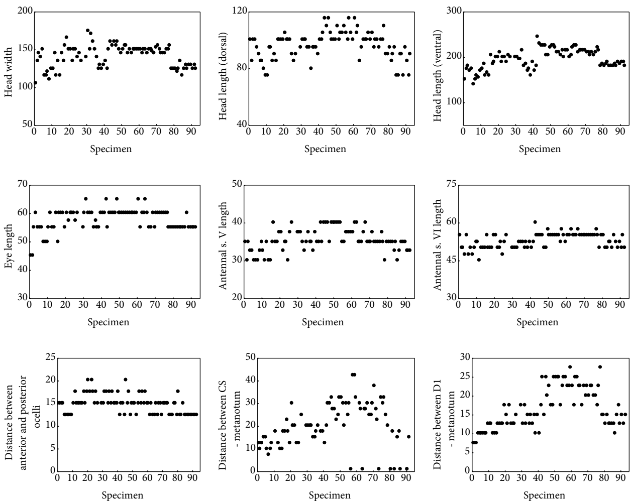
Figure 2a. Graphical visualization of characters 1–9. Axis x: 1–42 Thrips fuscipennis ; 43–93 T. sambuci (length in \mu\text{m} ).
