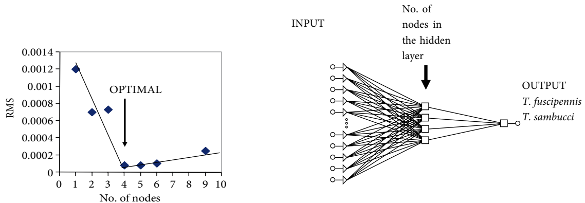
Figure 9. RMS as a function of the number of nodes in the hidden layer (left) and suggested optimal architecture (17, 4, 1).
