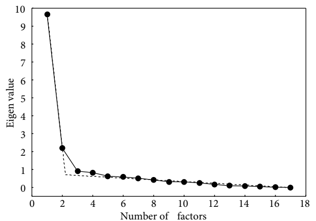
Figure 3. Plot of eigenvalues vs. number of eigenvalues factors.
