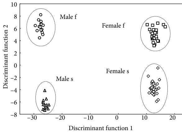
Figure 8. Linear discriminant analysis applied to distinguish T. fuscipennis – f and T. sambuci – s males and females.
