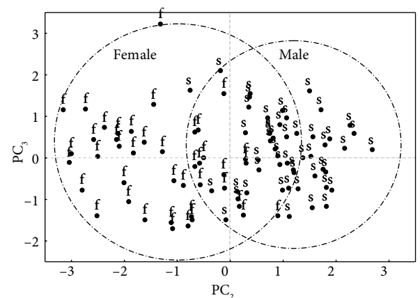
Figure 7. Graph of the principal components PC_2 vs. PC_3 concerning Thrips data analysis. f - T. fuscipennis ; s - T. sambuci .
