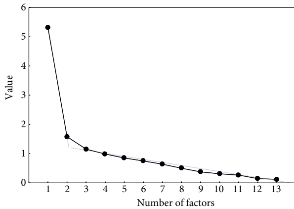
Figure 4. Eigenvalue analysis for T. fuscipennis and T. sambuci including females only; main variability is just given by 2 species, not by sex.
