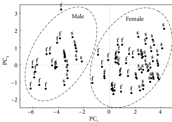
Figure 6. Graph of the principal components PC_1 vs. PC_3 concerning Thrips data analysis. f - T. fuscipennis ; s - T. sambuci .
