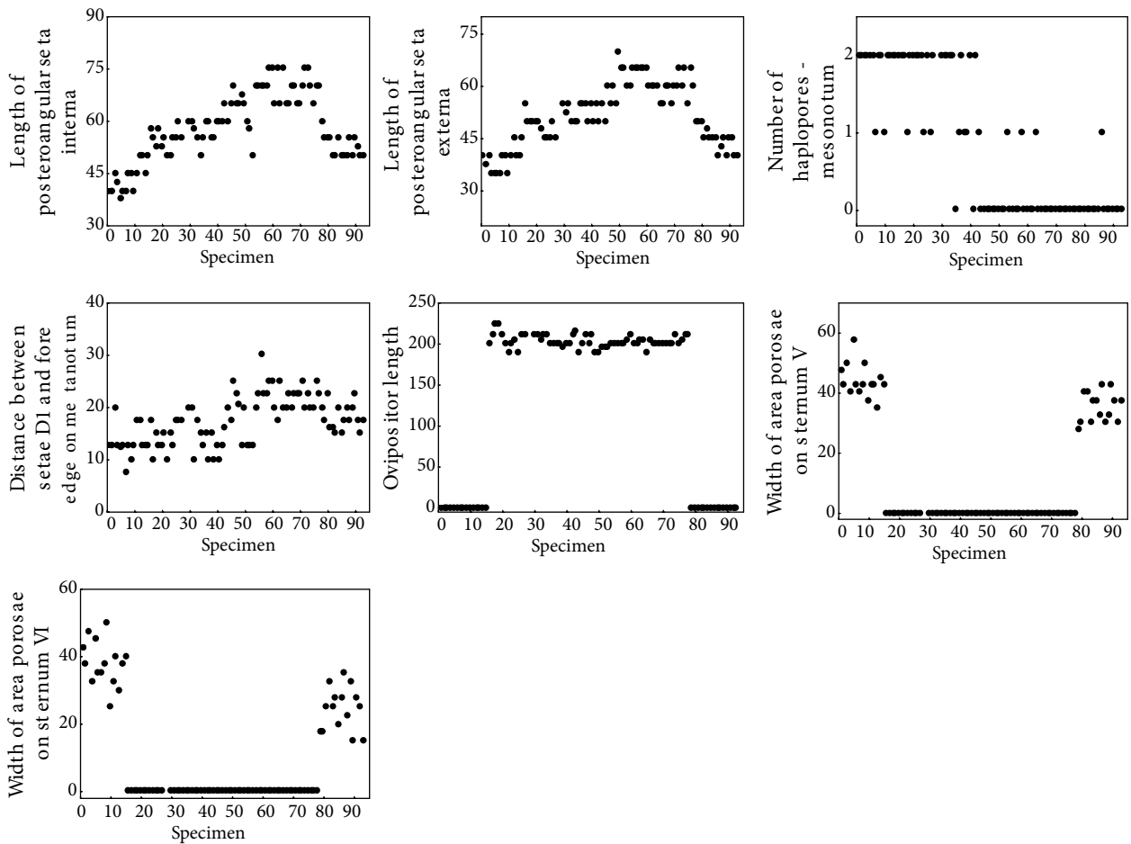
Figure 2b. Graphical visualization of characters 10–16. Axis x: 1–42 Thrips fuscipennis , 43–93 T. sambuci (length in \mu\text{m} ).
