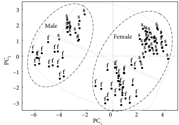
Figure 5. Graph of the principal components PC_1 vs. PC_2 concerning Thrips data analysis. f - T. fuscipennis ; s - T. sambuci .
